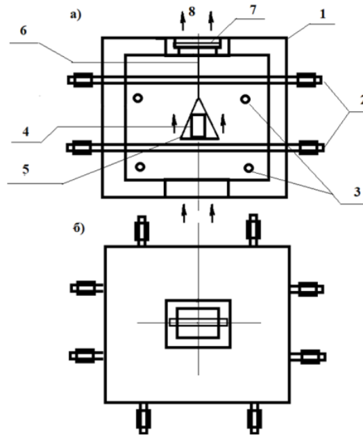
a) sectional melting devices: 1 — insulating housing; 2 and 3 — heaters; 4 — initial workpiece; 5 — substrate (platinum) with workpiece; 6 — substrate holder; 7 — ceramic rod for hanging the substrate; 8 — convection air flow; b) top view of the melting device
